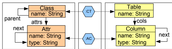
Figure 1: Triple type graph for CD2RDBM
